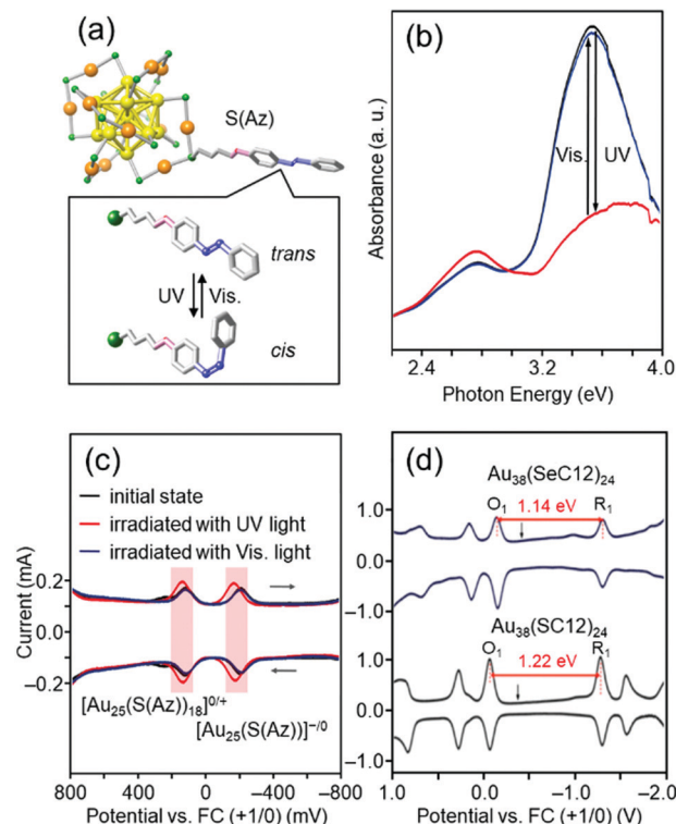
Fig. 8 (a) Proposed geometric structure of [Au_{25}(S(Az))_{18}]^- and (b) the photoresponsive behavior in the optical absorption spectra of [Au_{25}(S(Az))_{18}]^- in toluene solution in the energy range 2.2–4.0 eV. 122 The visible photostationary state (blue line) overlaps with the initial state (black line). (c) Photoresponse of the differential pulse voltammetry (DPV) curve of [Au_{25}(S(Az))_{18}]^- . 122 (d) DPV curves of [Au_{38}(SeC12)_{24}]^0 and [Au_{38}(SC12)_{24}]^0 in CH_2Cl_2 containing 0.1 M (C_4H_9)_4NClO_4 . 126 O_1 and R_1 indicate the first oxidation and reduction peaks of the NCs, respectively. The black arrows indicate the solution open-circuit potentials. The red arrows indicate the electrochemical HOMO–LUMO gaps of [Au_{38}(SeC12)_{24}]^0 and [Au_{38}(SC12)_{24}]^0 . Reproduced with permission from ref. 122 and 126. Copyright 2012 The Royal Society of Chemistry and 2013 American Chemical Society.
