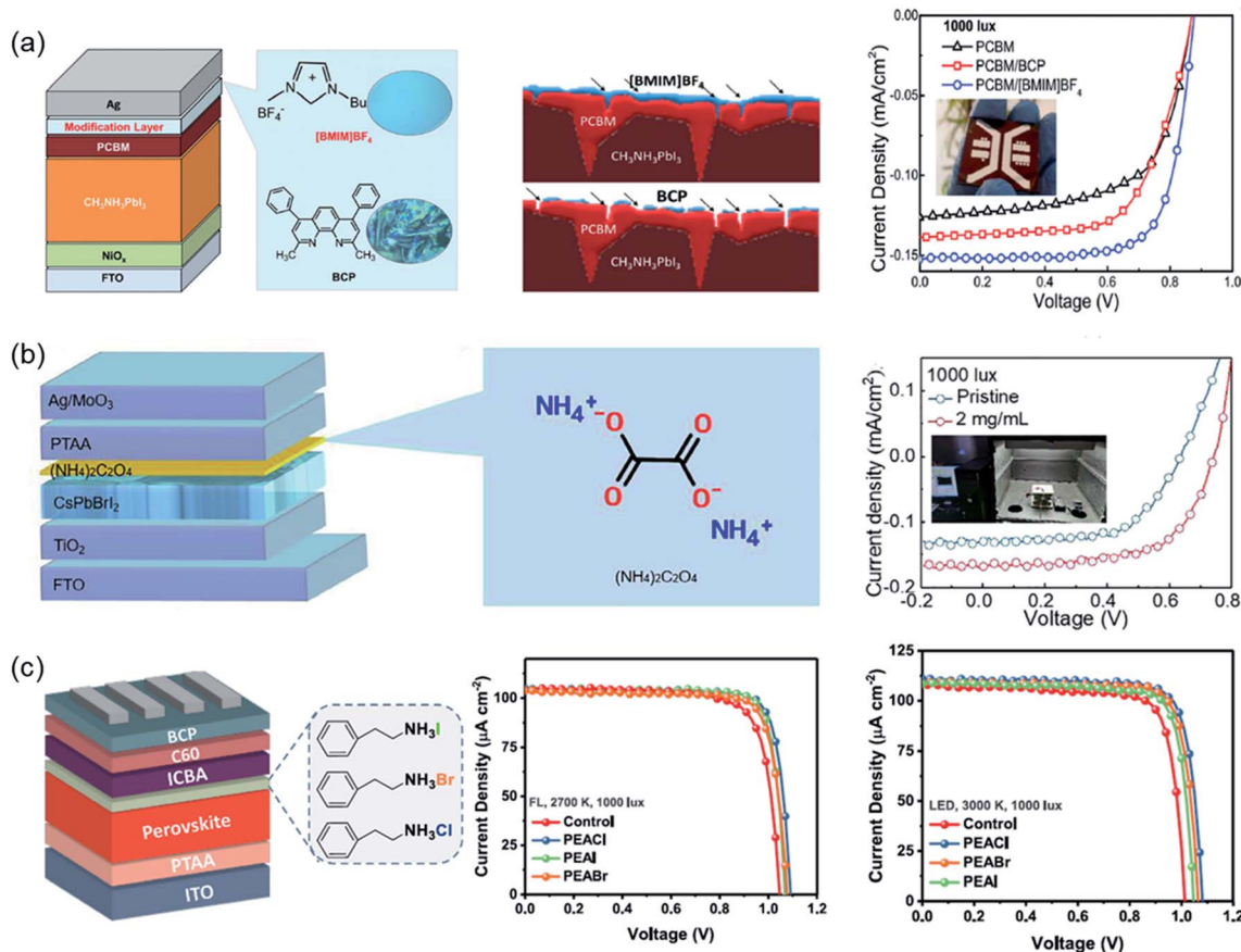
Fig. 6 (a) Inverted structure PSCs, molecular structure of [\text{BMIM}]\text{BF}_4 and BCP and the J-V curves. Reproduced from ref. 213 with permission from the [Wiley-VCH], copyright [2018]. (b) Device structure of \text{CsPbBrI}_2 based PSCs, molecular structure of (\text{NH}_4)_2\text{C}_2\text{O}_4 , and the J-V curves of devices with/without treatment. Reproduced from ref. 215 with permission from the [Elsevier], copyright [2020]. (c) Schematic diagram of PIPVs, the chemical structures of PEACl, PEABr, PEAI, and the J-V curves of the device with/without treatment under CFL and LED irradiation. Reproduced from ref. 216 with permission from the [Elsevier], copyright [2020].
