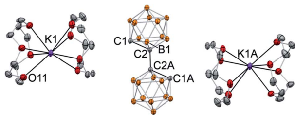
Fig. 5 Displacement ellipsoid plot (50% probability) of [\text{K}(12\text{-crown-}4)_2]_2(\text{C}_2\text{B}_{10}\text{H}_{10})_2 \cdot 4(\text{THF}) (6). Note the lack of \text{C}\cdots\text{K} contact and the complete ion separation. Only a half of the asymmetric unit is shown. Hydrogen atoms on boron atoms of the cluster and carbon atoms of the crown ether ligand have been omitted for clarity. Crystallization solvent molecules (THF) are not shown. Selected interatomic distances (Å): \text{K1}\cdots\text{C1} = 6.283(1) , \text{C1}-\text{C2} = 1.712(1) , \text{C1}-\text{B1} = 1.724(2) , \text{C2}-\text{B1} = 1.698(2) , \text{C2}-\text{C2A} = 1.532(2) Å.
