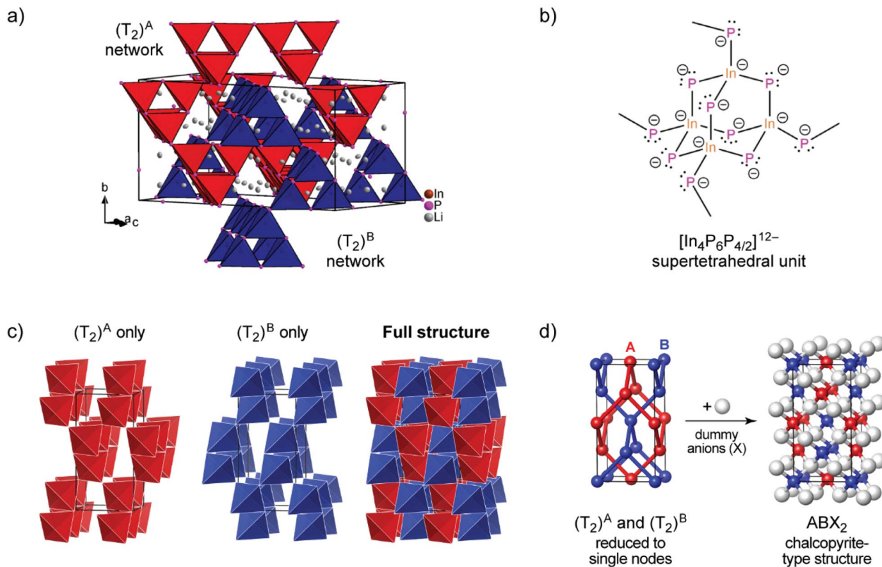
Fig. 1 (a) The crystal structure of \text{Li}_3\text{InP}_2 . The T2-supertetrahedra consist of four \text{InP}_4 tetrahedra and form two independent adamantane-like networks (the two networks, denoted as (\text{T}_2)^{\text{A}} and (\text{T}_2)^{\text{B}} , are shown in red and blue color, respectively). \text{Li}^+ ions are located in tetrahedral voids of the distorted ccp of P atoms. Li, In and P atoms are depicted in grey, brown and purple color, respectively (displacement ellipsoids set at 90% at 150 K). Crystal data and structure refinement are shown in Tables S1–S4 in the ESI.† CSD 2026514 contains the ESI crystallographic data for this paper.† (b) Lewis structure with formal charges of the atoms. (c) The two independent adamantane-like supertetrahedral networks (\text{T}_2)^{\text{A}} and (\text{T}_2)^{\text{B}} and the penetration of the two networks (each \text{T}_2 unit is represented by a tetrahedron). (d) A simplified view of the structure, in which the center of gravity of each \text{T}_2 unit is represented by a colored sphere (“node”), inspired by ref. 18 Notice: the \text{ABX}_2 chalcopyrite structure type is formed by the formal insertion of X atoms shown as grey spheres. Structural drawings in panels (c) and (d) were created using VESTA. 19
