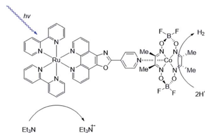
Fig. 21 This dye-HEC assembly sparked interest into supramolecular assemblies for proton reduction.
