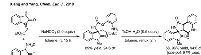
Scheme 46 Selected example of the combination of strategy B and C, using a nucleophilic C3 oxindole substituent and 3-ylidene oxindole.
