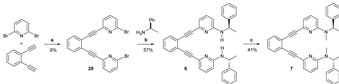
Scheme 5 The synthetic route to ligands 6 and 7 . Reagents and conditions: (a) Pd(PPh 3 ) 2 Cl 2 , CuI, NEt 3 , 110 °C, o.n.; (b) Pd 2 (dba) 3 , 1,3-bis(diphenylphosphino)propane, NaOtBu, ( R )-(+)-1-phenylethylamine, toluene, 90 °C, 3 h; (c) 1. NaH, DMF, r.t., 1 h, 2. MeI, DMF, r.t., 1 h, 3. NaH, DMF, r.t., 1 h, 4. MeI, DMF, r.t., 1 h. For details, see the ESI.†
