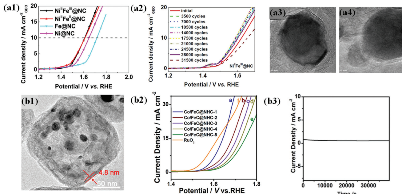
Fig. 9 (a1) LSV curves ( 10 \text{ mV s}^{-1} @ 900 \text{ rpm} ) of \text{Ni}^{\text{II}}\text{Fe}^{\text{III}}\text{@NC} , \text{Ni}^{\text{II}}\text{Fe}^{\text{II}}\text{@NC} , \text{Fe}_2[\text{Fe}^{\text{II}}(\text{CN})_6]_3 derived \text{Fe@NC} and \text{Ni}^{\text{II}}[\text{Ni}^{\text{II}}(\text{CN})_4] derived \text{Ni@NC} catalysts in oxygen-saturated 0.1 \text{ M KOH} solutions. (a2) LSV curves of \text{Ni}^{\text{II}}\text{Fe}^{\text{III}}\text{@NC} after a certain number of ADT cycles between 1.2 and 1.9 \text{ V} at 500 \text{ mV s}^{-1} . TEM images of (a3) \text{Ni}^{\text{II}}\text{Fe}^{\text{III}}\text{@NC} and (a4) \text{Ni}^{\text{II}}\text{Fe}^{\text{III}}\text{@NC} catalysts after ADT, reproduced with permission from ref. 63, Elsevier copyright 2017. (b1) TEM images of (A) \text{Co/FeC@NHC-1} (b2) OER polarization curves of \text{Co/FeC@NHC-1} , \text{Co/FeC@NHC-2} , \text{Co/FeC@NHC-3} , \text{Co/FeC@NHC-4} , \text{Co/FeC@NHC-5} , and \text{RuO}_2 in 1 \text{ M KOH} . (b3) Potentiostatic response (current density versus time) under a constant potential of 1.54 \text{ V vs. RHE} , reproduced with permission from ref. 151, Elsevier copyright 2020.
