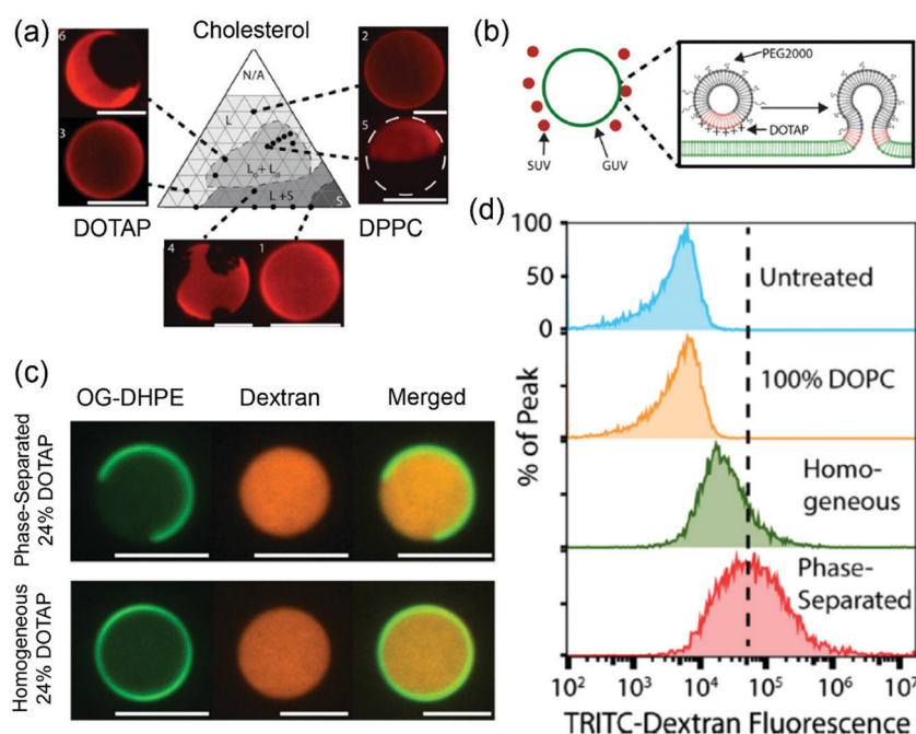
Fig. 6 (a) A DOTAP/DPPC/cholesterol phase diagram at 25 °C. Texas red–DPPE (0.3 mol%) was used to visualize different phases. (b) Schematic illustration of phase-separated DOTAP containing SUVs fusing to a GUV. (c) Confocal fluorescence micrographs of phase separated (24 mol% DOTAP, 38 mol% cholesterol, 36 mol% DPPC, 2 mol% PEG2000–DPPE) and homogeneous (24 mol% DOTAP, 74 mol% DOPC, 2 mol% PEG2000–DPPE) liposomes loaded with TRITC–dextran (red). The liposomes were labeled with 1 mol% Oregon green–DPPE (green). (d) Flow cytometry histograms of cells incubated with GUVs loaded with TRITC–dextran. Adapted with permission from ref. 123. Copyright © 2017 Biomedical Engineering Society.
