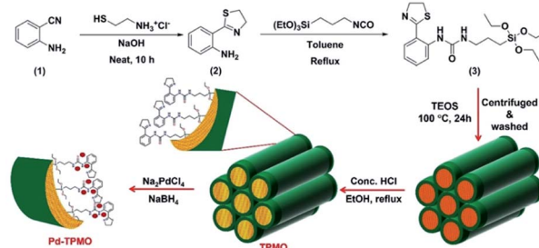
Fig. 38 Synthesis of the thiazoline-silyl precursor, thiazoline bridged periodic mesoporous organosilica (TPMO) and Pd NP entrapped TPMO (Pd-TPMO). 199 Reproduced with permission. 199 Copyright 2012, John Wiley & Sons.
