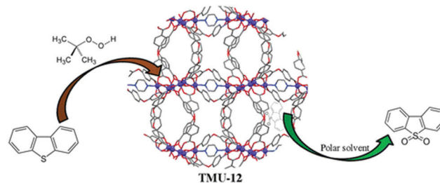
Fig. 17 Cobalt metal organic frameworks as catalysts in the oxidative desulfurization [reprinted with permission from ref. 177, Copyright © Royal Society of Chemistry, 2015].
