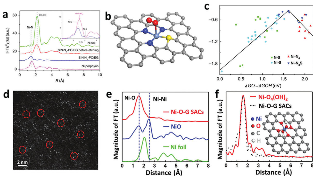
Fig. 18 (a) Fourier-transformed magnitudes of the experimental K-edge EXAFS signals of Ni-N 3 S SAC. (b) Structural geometry of Ni-N 3 S SAC with O-O bond. (c) OER volcano plot of the overpotential \eta vs. the difference between the adsorption free energy of \text{*O} and \text{*OH} for the N-S, Ni-S, Ni-N 4 , and Ni-N 3 S models. Reproduced with permission from ref. 353. Copyright 2019, Springer Nature. (d) Atomic-scale HAADF-STEM image of Ni-O 4 -G SACs. (e) FT-EXAFS spectra of Ni-O 4 -G SACs with NiO and Ni foil references. (f) FT-EXAFS data of the proposed Ni-O 4 (OH) 2 architecture compared to experimental Ni-O 4 . Reproduced with permission from ref. 354. Copyright 2020, Wiley VCH.
