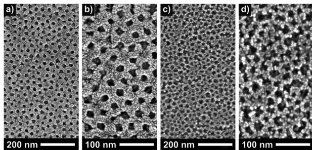
Fig. 3 Top-view SEM images of sol-gel-derived (a and b) and preformed nanoparticle-based (c and d) mesoporous TiO 2 thin films. Reproduced from ref. 20 with permission.
