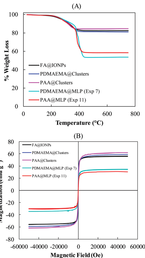
Fig. 7 (A) TGA and (B) SQUID analyses of the commercial fatty acid-modified IO nanoparticles (FA@IONPs), the PDMAEMA@clusters, the PAA@clusters, and the magnetic fraction ( \omega_{\text{mag}} ) of the PDMAEMA@MLP and PAA@MLP samples (Exp. 7, Table 1 and Exp. 11, Table 2).
