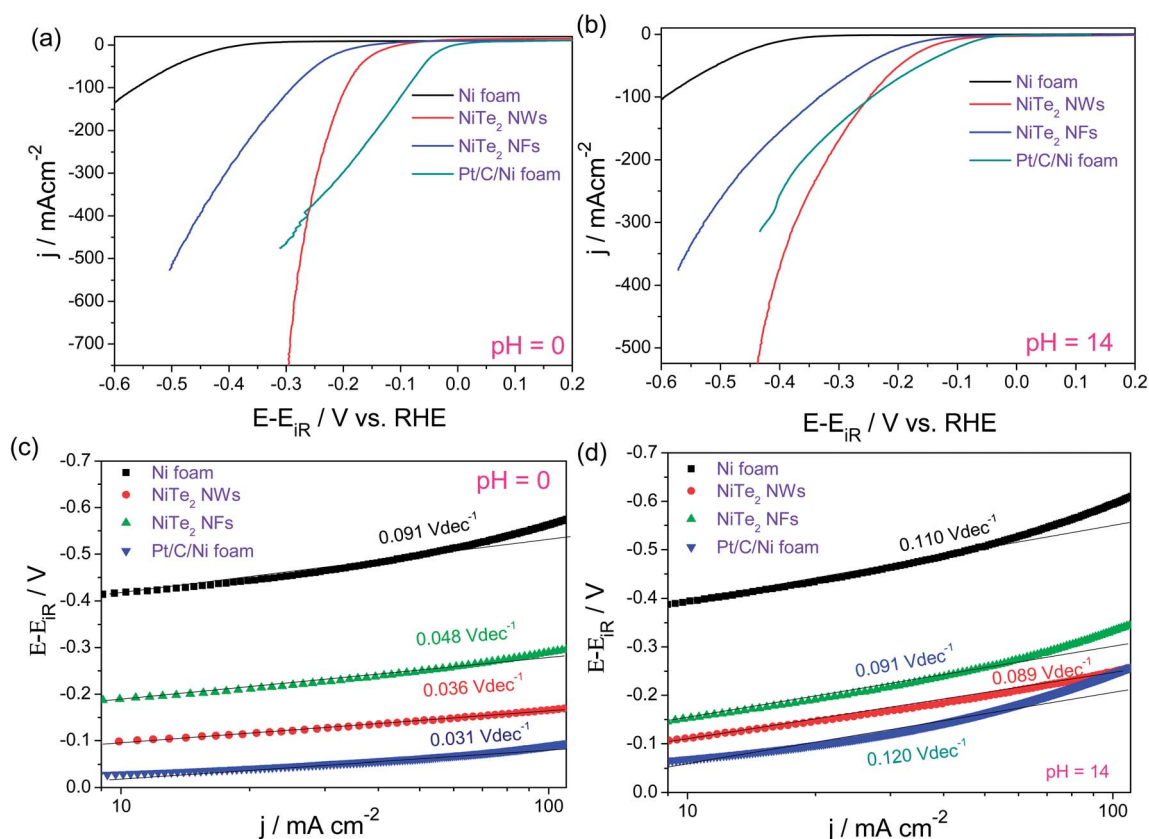
Fig. 12 (a and b) HER LSVs of \text{NiTe}_2 NWs, \text{NiTe}_2 NFs, Ni foam and Pt/C–Ni foam in 0.5 M \text{H}_2\text{SO}_4 and 1.0 M KOH, respectively (sweep rate – 5 \text{mV s}^{-1} ). (c and d) Tafel plots of the same. Reproduced with permission from ref. 91 (Copyright 2018 American Chemical Society).
