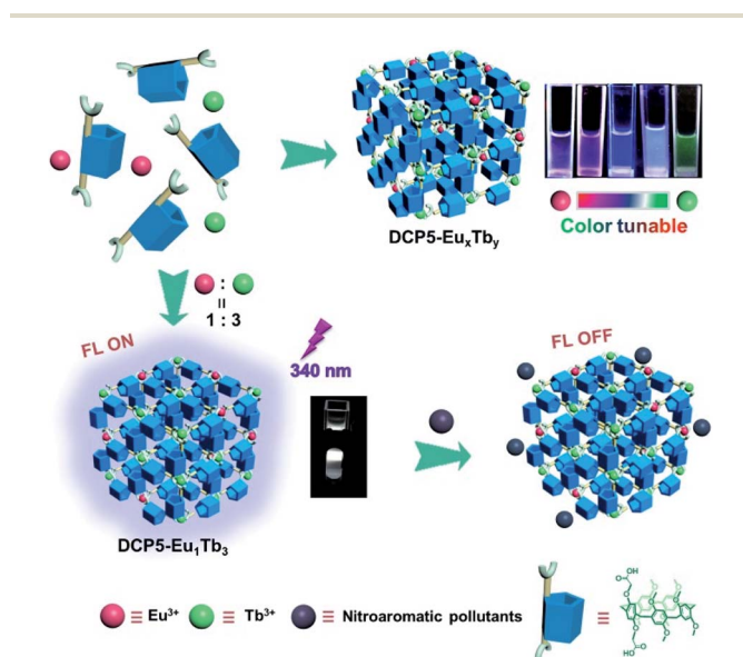
Fig. 1 Schematic illustration of the construction of the color-tunable pillarene coordination polymer (PCP), i.e. , DCP5- \text{Eu}_x\text{Tb}_y , simply by tuning the molar ratio of \text{Eu}^{3+} and \text{Tb}^{3+} in the system and the fluorescence ON/OFF sensing of nitroaromatic pollutants by a typical PCP, i.e. , DCP5- \text{Eu}_1\text{Tb}_3 .
