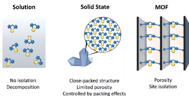
Fig. 1 A schematic showing a comparison of the chemical environment of reactive metal complexes in solution, in the solid-state as a typical molecular crystal, and isolated in a MOF support.
