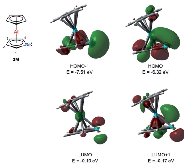
Fig. 5 Calculated surface diagrams of frontier molecular orbitals of germaaluminocene 3M (M06-2X/6-311+G(d,p), isodensity value 0.04).
