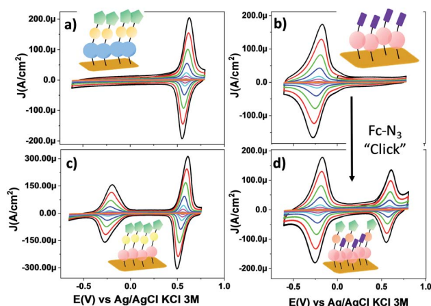
Fig. 4 CV curves of SAMs on gold: (a) SAM-3-H , (b) SAM-2-Rad , (c) SAM-3-Rad and (d) SAM-5-Rad in \text{CH}_2\text{Cl}_2 + 0.2 M \text{Bu}_4\text{NPF}_6 at different scan rates ( 0.05 , 0.1 , 0.25 , 0.5 , 1 , 2 , 3 and 4 \text{V s}^{-1} ). The color code used for SAMs is the same as that used in Scheme 1. (Blue) PTM \alpha\text{H} ; (magenta) PTM radical; (yellow) triazole ring; (green) Fc and (violet) terminal alkyne moieties.
