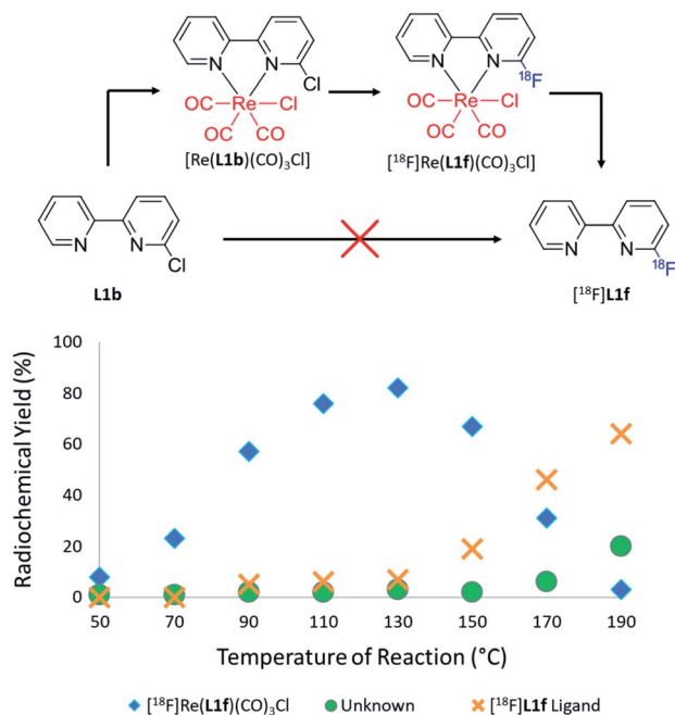
Fig. 3 [\text{18F}]\text{Fluoride} substitution in the ortho position of [\text{Re}(\text{L1b})(\text{CO})_3\text{Cl}] which afforded [\text{18F}][\text{Re}(\text{L1f})(\text{CO})_3\text{Cl}] (blue diamonds). Thermal decomplexation led to the subsequent formation of [\text{18F}]\text{L1f} (orange crosses) and an unknown by-product (green circles) with the RCYs plotted as a function of reaction temperature. [\text{18F}]\text{L1f} was unable to be synthesised from \text{L1b} without first complexing to a rhenium(i) centre.
