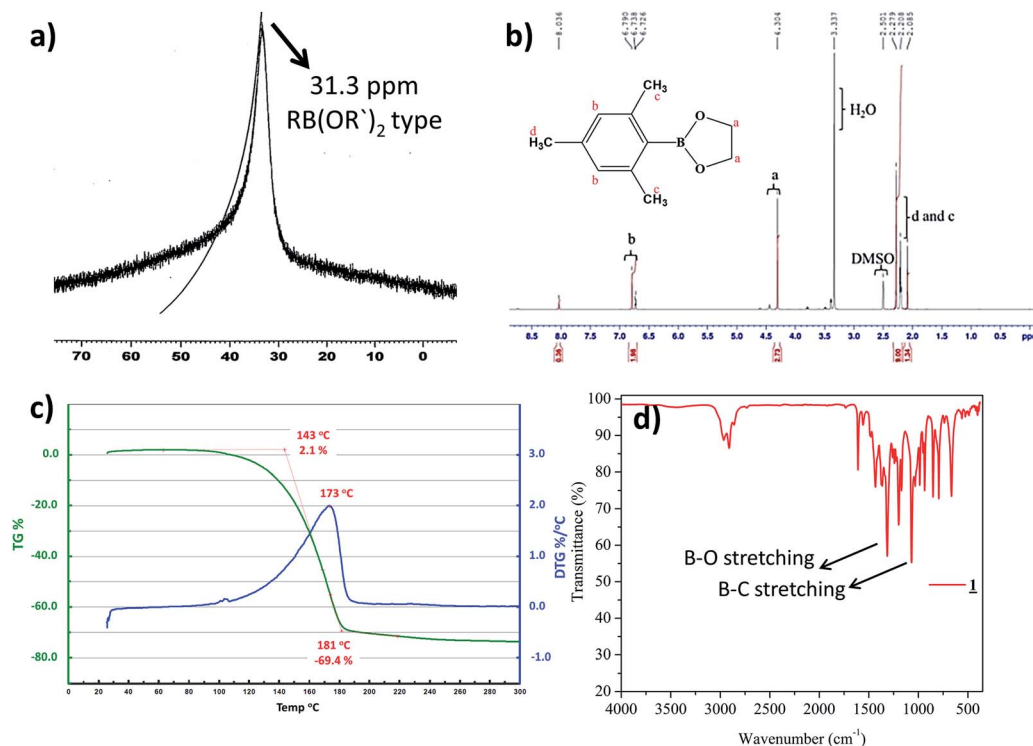
Fig. 2 (a) 11 B-NMR of 1 in DMSO- d 6 , (b) 1 H-NMR of 1 in DMSO- d 6 (c) TGA profile of 1 (d) IR Spectrum of 1 .
