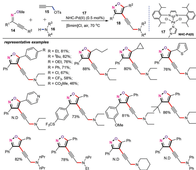
Scheme 7 Palladium-catalyzed three-component cascade cyclization/alkynylation.
