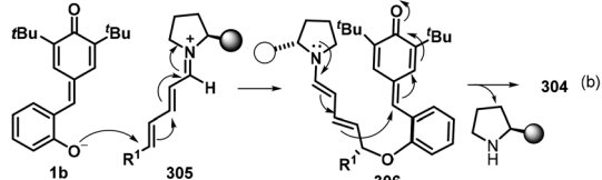
Scheme 66 Double 1,6-addition for the synthesis of chiral chromans.
