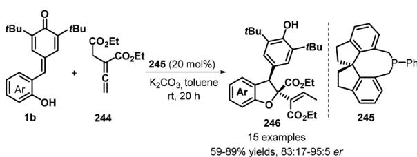
Scheme 54 Enantioselective catalytic [4 + 1]-cyclization of p -QMs with allenates.
