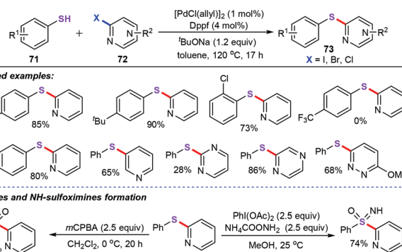
Scheme 28 Palladium-catalyzed thioetherification of thiols and 2-chloroheteroaromatics.
