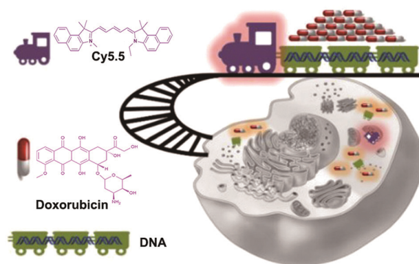
Fig. 15 Schematic of the MitoDNATrs delivery system. Reproduced with permission from ref. 118. Copyright 2019, American Chemical Society.
