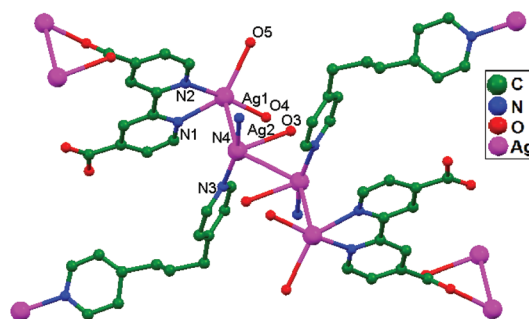
Fig. 36 The coordination environment of \text{Ag}^+ ions in 58 ; free water molecules and hydrogen atoms have been omitted.
