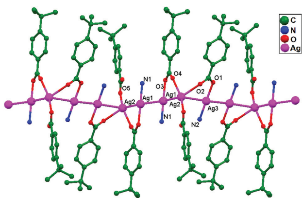
Fig. 44 The 1D silver wire incorporating ligand-supported and unsupported Ag–Ag contacts in 72.
