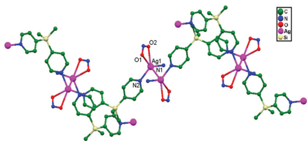
Fig. 20 The coordination environment around \text{Ag}^+ ions, with ligand-unsupported argentophilic interactions forming a zigzag chain in [\text{Ag}(\text{NO}_2)(\text{BPDMS})]_2 , 31 .
