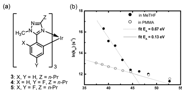
Fig. 6 (a) Chemical structures of 3–5 and (b) Arrhenius (activation energy) plot of 5 dissolved in 2-MeTHF or solid PMMA host. Adapted with permission from ref. 81. Copyright 2008, Elsevier.
