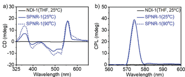
Fig. 4 (a) CD and (b) CPL spectra of NDI-1 in THF ( c = 0.35\text{ mM} ) and SPNR-1 in water (NDI-1 concentration = 0.34\text{ mM} ; l = 0.1\text{ cm} ). Molar ellipticity at \lambda_{\text{max}} for SPNR-1 ( 25\text{ }^\circ\text{C} ) was estimated to be 5.36 \times 10^5\text{ M}^{-1}\text{ cm}^{-1} from the CD spectrum.
