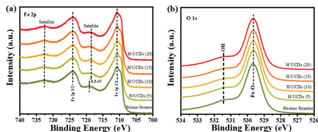
Fig. 4 (a) High resolution XPS of Fe 2p line, (b) High resolution XPS of O 1s line for pristine hematite and H/UCDs photoanodes.
