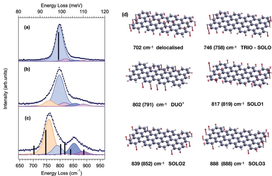
Fig. 2 Comparison between HREEL spectrum of 7-aGNR grown in different conditions, i.e. different substrate deposition temperature T_D and coverage \theta_{ML} : (a) T_D = 200\text{ °C} \theta_{ML} = 0.26 ; (b) T_D = RT \theta_{ML} = 0.33 (also depicted in the right panel of Fig. 1); (c) T_D = 310\text{ °C} \theta_{ML} = 0.42 . Blue dots represent experimental data, solid black lines are the respective fitting curves, whereas the fitting components are reported (with a small downward shift for the sake of clarity) as shaded curves. The intensity and frequency of the calculated Z-polarized IR-active modes of the 7-aGNR dimer and of the infinite 7-aGNR are reported as black bars in panel (a) and (c), respectively. The corresponding atomic displacements for the dimer are reported in panel (d), where the direction and magnitude of the displacement for each atom involved in the vibration are represented by red vectors. Experimental frequencies, as determined by the fitting procedure, are reported in parenthesis, for comparison.
