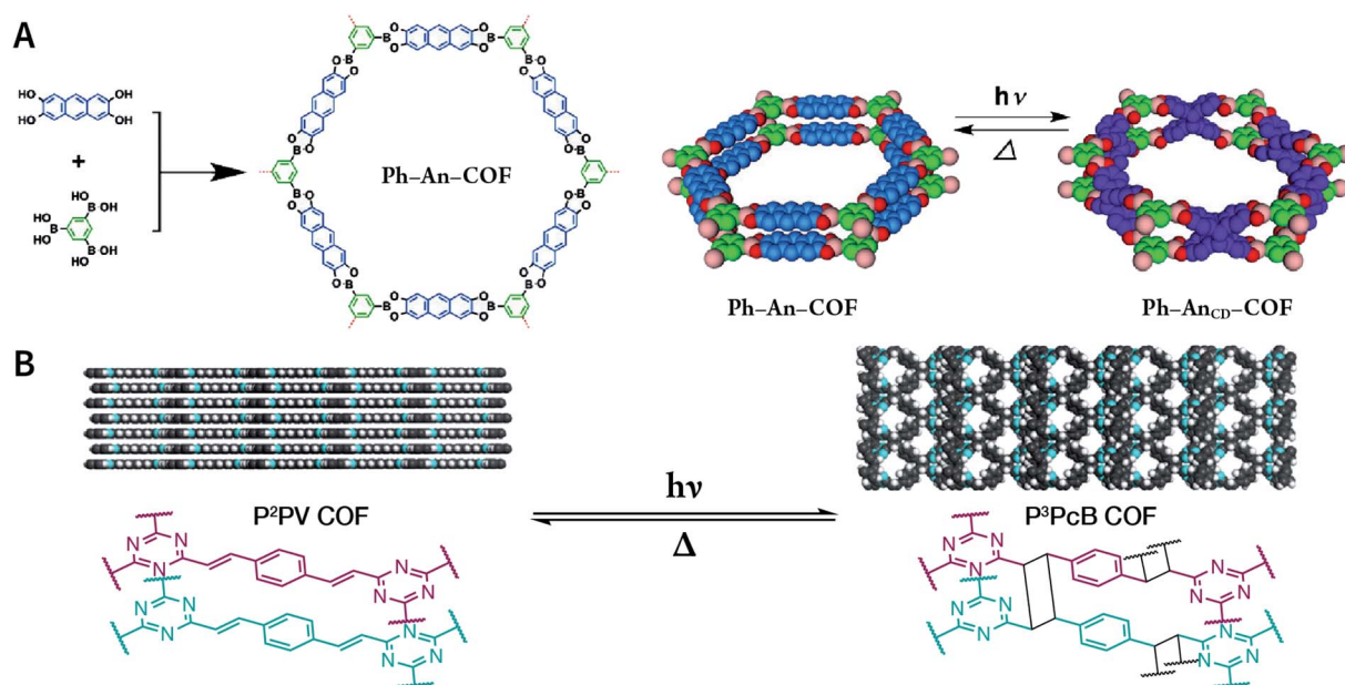
Fig. 62 (A) Reversible interlayer [4 + 4] cycloaddition reaction of anthracene-based Ph-An-COF. Adapted under a Creative Commons Attribution Non-Commercial License. Copyright 2015, The Author(s). 347 Published by Wiley-VCH Verlag GmbH & Co. KGaA, Weinheim. (B) Partially reversible interlayer [2 + 2] cycloaddition reaction of vinylene-linked P 2 PV COF. Adapted with permission. 350 Copyright 2020, American Chemical Society.
