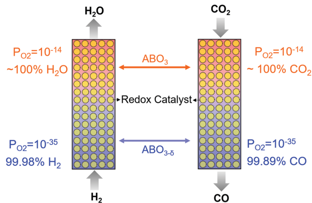
Fig. 7 RWGS in a counter-currently operated two-step chemical looping scheme using ABO_3 perovskite as a redox catalyst at 500 °C.
