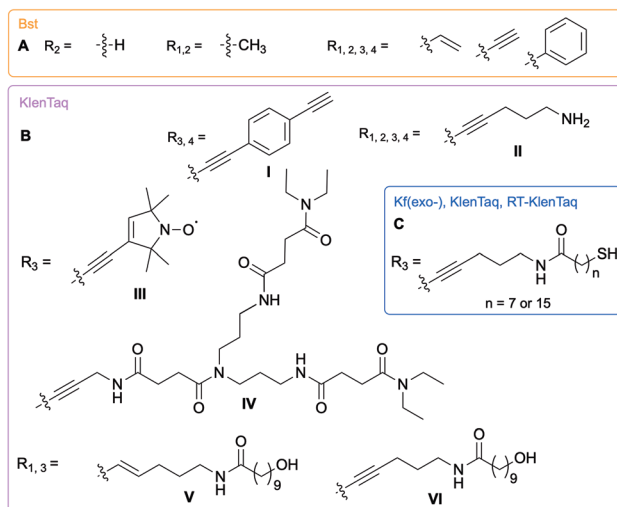
Fig. 2 Structures of nucleobase alterations of nucleobase-modified dNTPs oriented towards the major groove of DNA for investigating bacterial polymerase activity.
