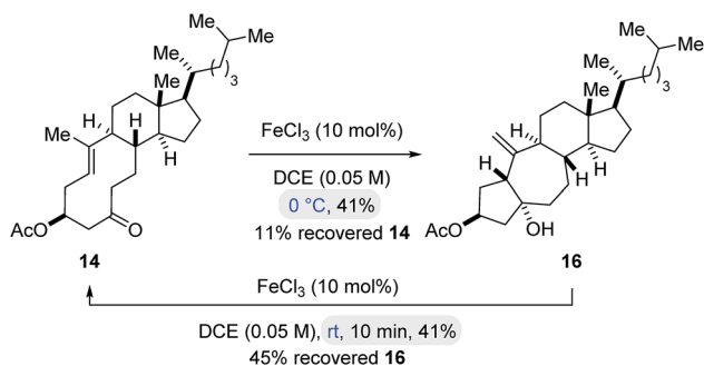
Scheme 2 FeCl 3 also catalyses a reversible transannular carbonyl-ene reaction.
