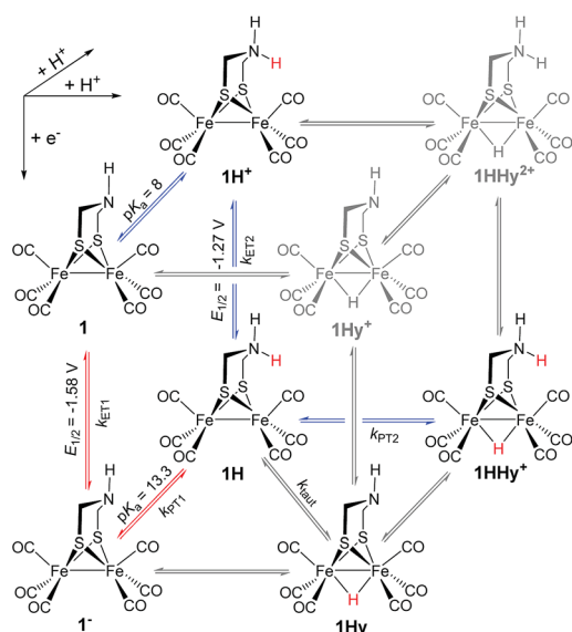
Scheme 2 Metal and ligand protonation reactions of 1 (Fe 2 ( adt )(CO) 6 ) and 1 - (Fe 2 ( adt )(CO) 6 ) - .
