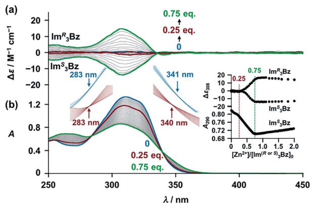
Fig. 1 (a) CD spectra of \text{Im}^R_3\text{Bz} and \text{Im}^S_3\text{Bz} (concentrations: 2.0 \times 10^{-5} M) in the presence of \text{Zn}^{2+} [0 (blue), 5.0 \times 10^{-6} (red) and 1.5 \times 10^{-5} M (green)] in acetonitrile at 298 K, where \Delta\epsilon is calculated based on the ligand concentration ( 2.0 \times 10^{-5} M). (b) Corresponding UV/vis absorption spectral changes observed in the titration of \text{Im}^S_3\text{Bz} by \text{Zn}^{2+} . Inset: plots of \Delta\epsilon at 308 nm absorbance at 290 nm versus [\text{Zn}^{2+}]/[\text{Im}^{(R \text{ or } S)}_3\text{Bz}]_0 . The magnified spectra around the isosbestic points (blue lines: [\text{Zn}^{2+}] = 0\text{--}5.0 \times 10^{-6} M; red lines: 5.0 \times 10^{-6} M to 1.5 \times 10^{-5} M). For clarity reasons two step spectral changes are separated vertically.
