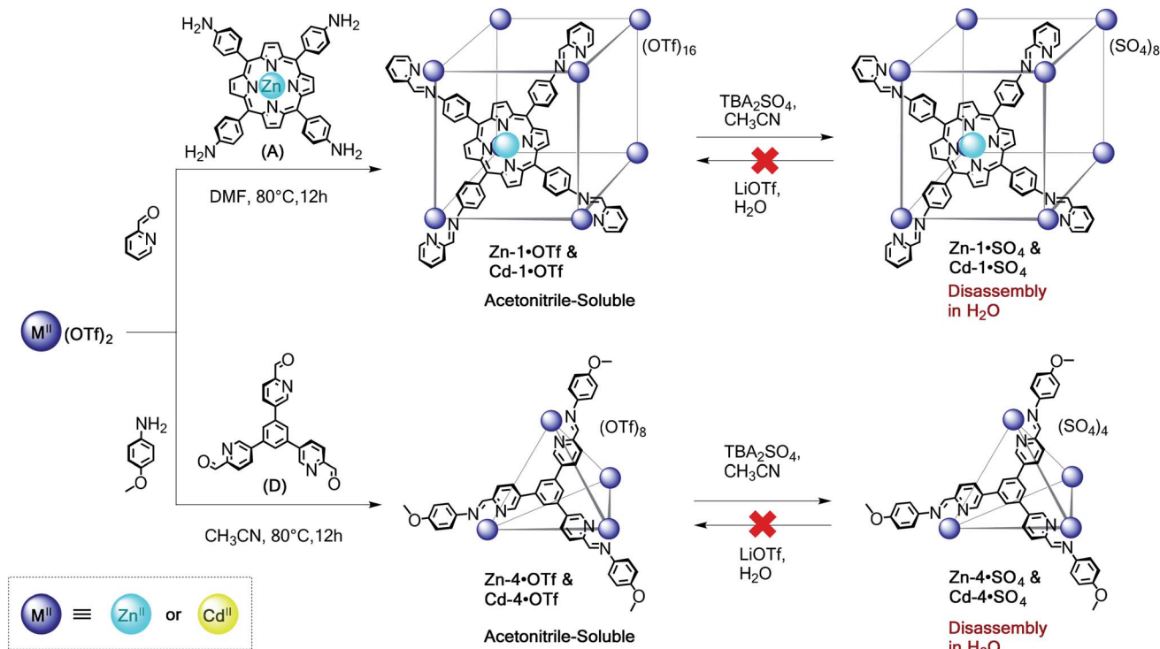
Scheme 4 Self-assembly of face-capped cubic 1 and tetrahedral 4 architectures based on zinc(II) and cadmium(II). Sulfate salts of capsules obtained via anion exchange from the triflate congeners were observed to disassemble in water. Direct assembly reactions using ZnSO_4 or CdSO_4 did not form the target water-soluble products.
