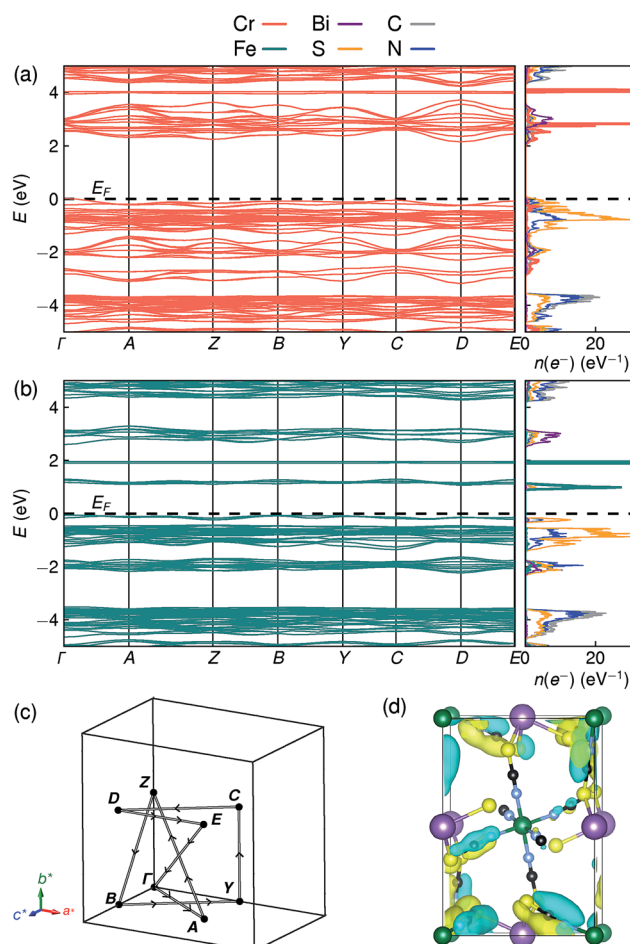
Fig. 6 DFT calculated band structure and element-projected density of states for (a) Cr[Bi(SCN)_6] and (b) Fe[Bi(SCN)_6] . Both spin channels have been plotted at once, as the differences between them are minor. (c) Reciprocal space path used for band structure calculations. (d) Kohn–Sham orbital for Cr[Bi(SCN)_6] at the valence band maximum, showing the localised nature of the valence band states, viewed along the [100] direction. Atoms are coloured as in Fig. 3.
