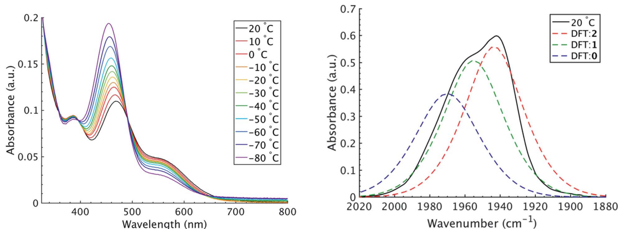
Fig. 4 (Left) VT-UV-vis spectroscopy in DCM ranging from 20 to -80 °C. The absorbance maximum at 470 nm is attributed to the apical isomer (2) while the maxima at 385 and 561 nm are attributed to the equatorial isomer (1). (Right) Predicted FTIR spectrum from DFT calculation. Experimental data at 20 °C is shown as the black trace, apical isomer shown as the red trace, equatorial isomer shown as green trace, and TBP isomer as blue trace.
