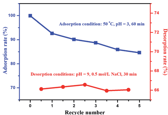
Fig. 8 Effect of the recycle number on adsorption and desorption.
