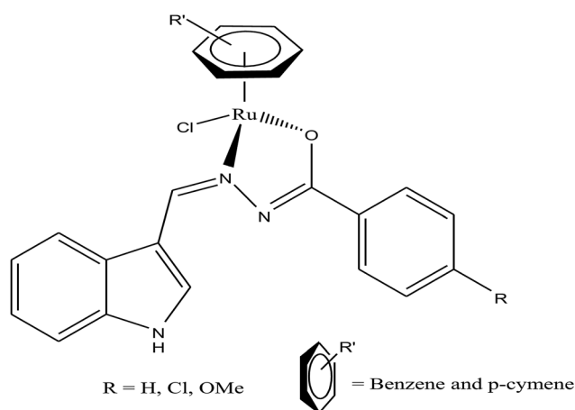
Fig. 4 Chemical structure of ruthenium(II) arene benzhydrazone complexes.
