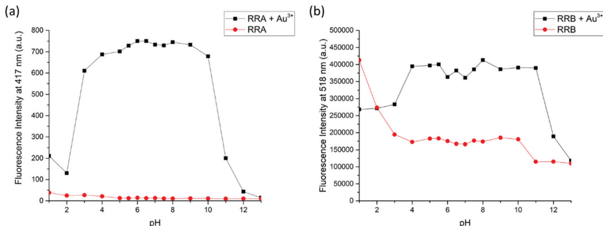
Fig. 7 (a) Fluorescence response of RRA (20 \mu\text{M} , \lambda_{\text{ex}} = 370 \text{ nm} ) at 417 nm upon addition of 10 equiv. of \text{Au}^{3+} in THF/MeCN/ \text{H}_2\text{O} solution (2 : 48 : 50, v/v/v) (pH 1–13) indicated by the black line; fluorescence of RRA at 417 nm in THF/MeCN/ \text{H}_2\text{O} solution (2 : 48 : 50, v/v/v) (pH 1–13) indicated by the red line. (b) Fluorescence response of RRB (5 \mu\text{M} , \lambda_{\text{ex}} = 500 \text{ nm} ) at 518 nm upon addition of 10 equiv. of \text{Au}^{3+} in MeCN/ \text{H}_2\text{O} solution (50 : 50, v/v) (pH 1–13) indicated by the black line; fluorescence of RRB at 518 nm in MeCN/ \text{H}_2\text{O} solution (50 : 50, v/v) (pH 1–13) indicated by the red line.
