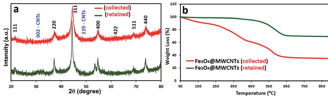
Fig. 5 (a) XRD patterns and (b) TGA curves for Fe 3 O 4 @MWCNT exiting (red) and retained (green) in the quartz tube, processed in the VFD (optimised parameters) operating at 8.5k rpm rotational speed, with the concentration of the as received MWCNTs at 0.08 mg mL -1 (DMF, tilt angle 45°, flow rate 0.45 mL min -1 , and laser power 250 mJ).
