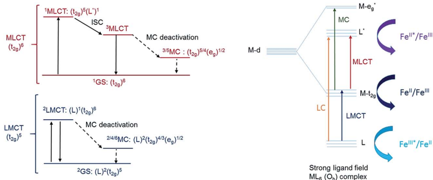
Fig. 2 Simplified Jablonski-type diagram for low-spin \text{Fe}^{\text{II}} 3d^5 and \text{Fe}^{\text{III}} 3d^6 complexes (left), together with a schematic illustration of key electronic levels and photoexcitation processes involved in the photophysics (right). Curved arrows indicate opportunities to drive subsequent bimolecular or interfacial electron transfer processes (far right).
