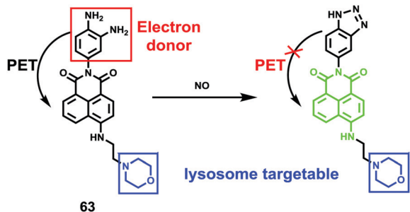
Scheme 49 Fluorescent probe 63 for NO.
