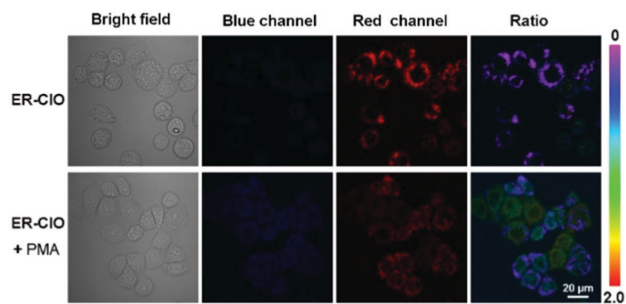
Fig. 4 Confocal fluorescence images of endogenous \text{ClO}^- by ER-CIO. HeLa cells were incubated with or without PMA at 37 °C for 30 min, and then further treated with ER-CIO (10 \mu\text{M} ) for another 30 min. For the blue channel: \lambda_{\text{ex}} = 403 \text{ nm} , \lambda_{\text{em}} = 425\text{--}475 \text{ nm} ; for the red channel: \lambda_{\text{ex}} = 488 \text{ nm} , \lambda_{\text{em}} = 552\text{--}637 \text{ nm} . The ratiometric images ( F_{\text{blue}}/F_{\text{red}} ) were obtained by merging the yellow channel image with the related red channel image. Scale bar: 20 \mu\text{m} .
