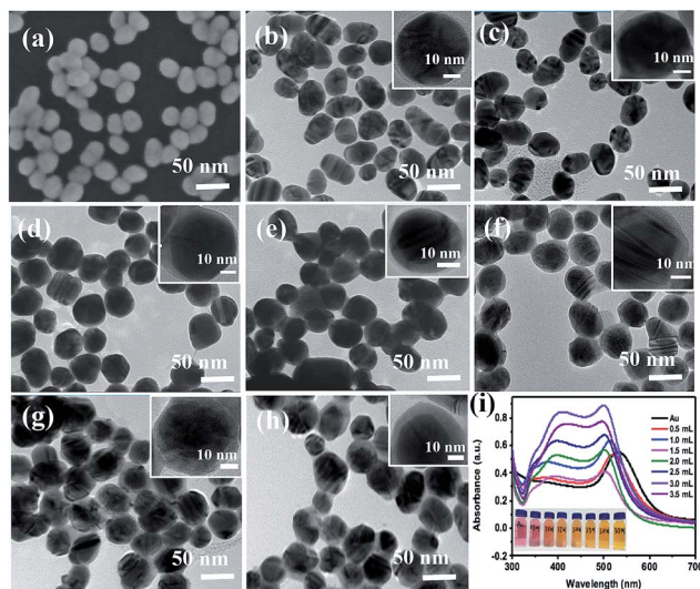
Fig. 2 (a) SEM image of Au NPs and (b–h) TEM images of the Au@Ag core-shell NPs synthesized under adding AgNO 3 in amounts from 0.50 to 3.50 mL at a gradient of 0.50 mL, respectively. The inset HRTEM images present the thickness of Ag shell from 1.0 to 10.0 nm; (i) the absorption spectra of Au NPs and Au@Ag core-shell NPs with the increase in the amount of AgNO 3 from 0.50 to 3.50 mL, the inset shows the colour of the solutions at different dosages of AgNO 3 solution.
