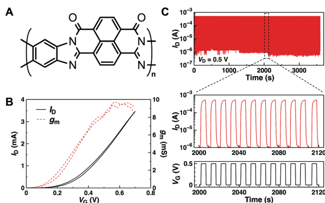
Fig. 4 (A) Chemical structure of BBL. (B) n-Type transfer curve (black) and transconductance (red dotted) of a 180 \text{ nm} -thick BBL OECT measured at V_D = 0.6 \text{ V} in 0.1 \text{ M NaCl} . (C) Stability test of BBL OECT under sequential square wave gate voltage pulse for 1 \text{ h} in water. Reprinted with permission from ref. 58 copyright The Authors.
