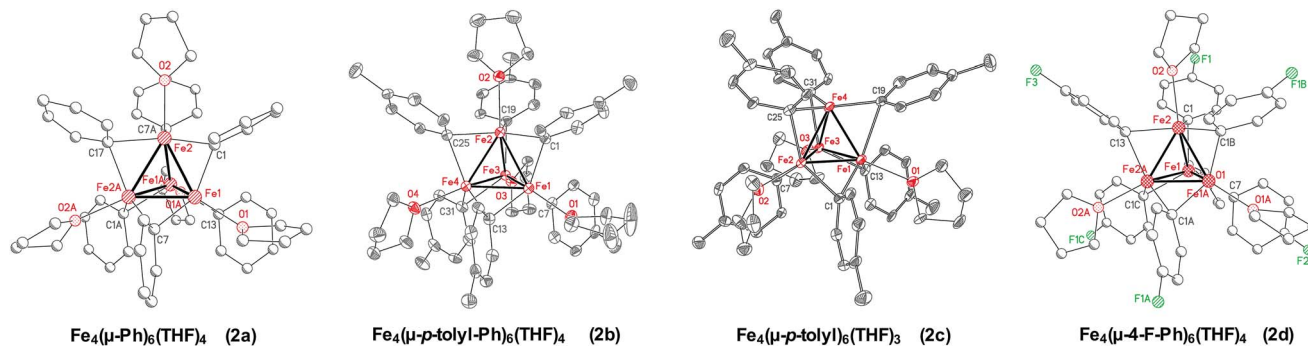
Fig. 3 Crystal structures of the tetranuclear iron–aryl clusters, with hydrogen atoms omitted for clarity. Due to weakly diffract crystals, the structures of \text{Fe}_4(\mu\text{-Ph})_6(\text{THF})_4 ( 2a ) and \text{Fe}_4(\mu\text{-4-F-Ph})_6(\text{THF})_4 ( 2d ) are used solely for connectivity and chemical formulation as shown. For structures with p -tolyl groups, \text{Fe}_4(\mu\text{-}p\text{-tolyl})_6(\text{THF})_3 ( 2b ) and \text{Fe}_4(\mu\text{-}p\text{-tolyl})_6(\text{THF})_4 ( 2c ), adequate intensity data could be obtained and the ellipsoids are shown at 50% probability.
