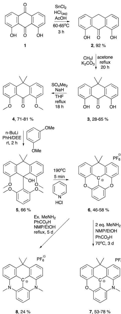
Scheme 1 Synthesis of the carbon-bridged dioxatriangulenium (6), azaoxatriangulenium (7), and diazatriangulenium salts (6, 7, and 8, respectively).
